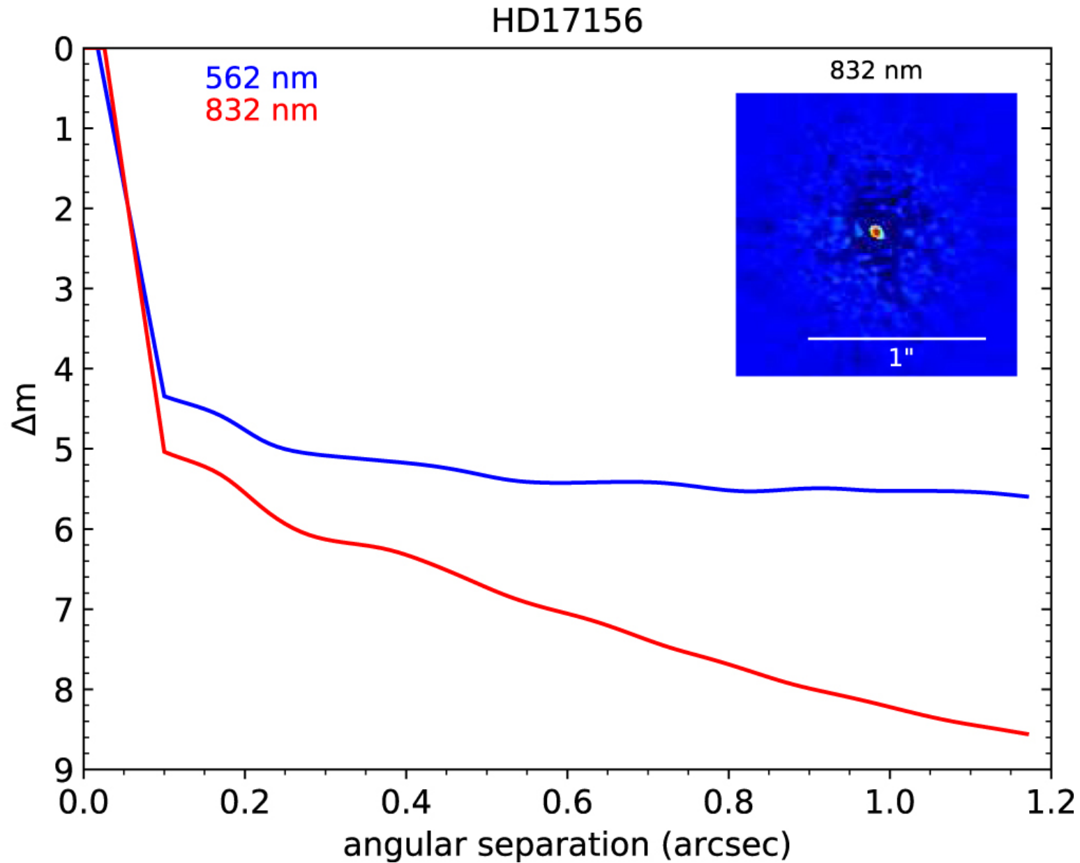
Figure 4. from Stephen R. Kane et al 2023 Astron. J. 165 doi:10.3847/1538-3881/acd17a https://dx.doi.org/10.3847/1538-3881/acd17a © 2023. The Author(s). Published by the American Astronomical Society.
