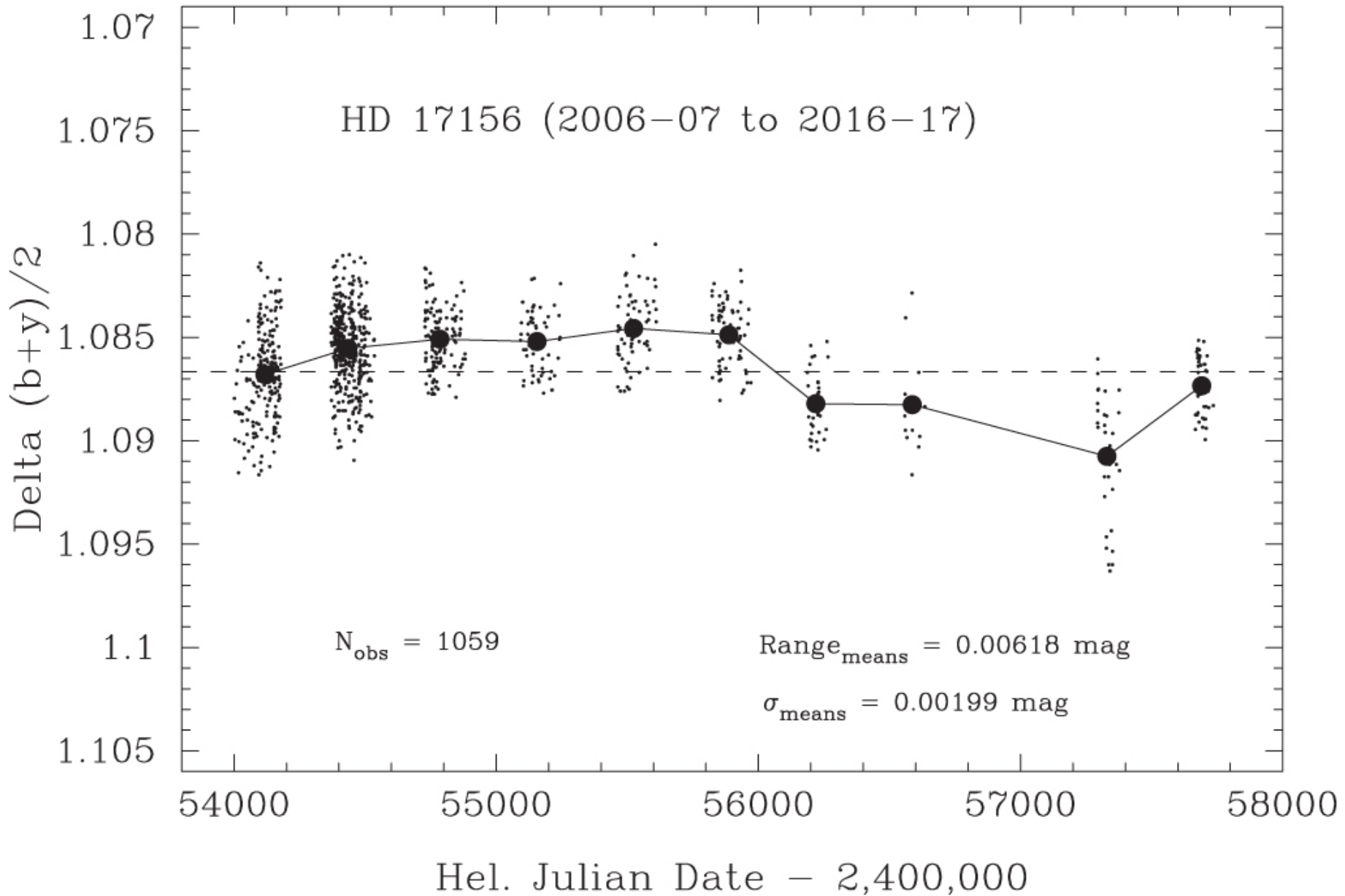
Figure 2. from Stephen R. Kane et al 2023 Astron. J. 165 doi:10.3847/1538-3881/acd17a https://dx.doi.org/10.3847/1538-3881/acd17a © 2023. The Author(s). Published by the American Astronomical Society.
