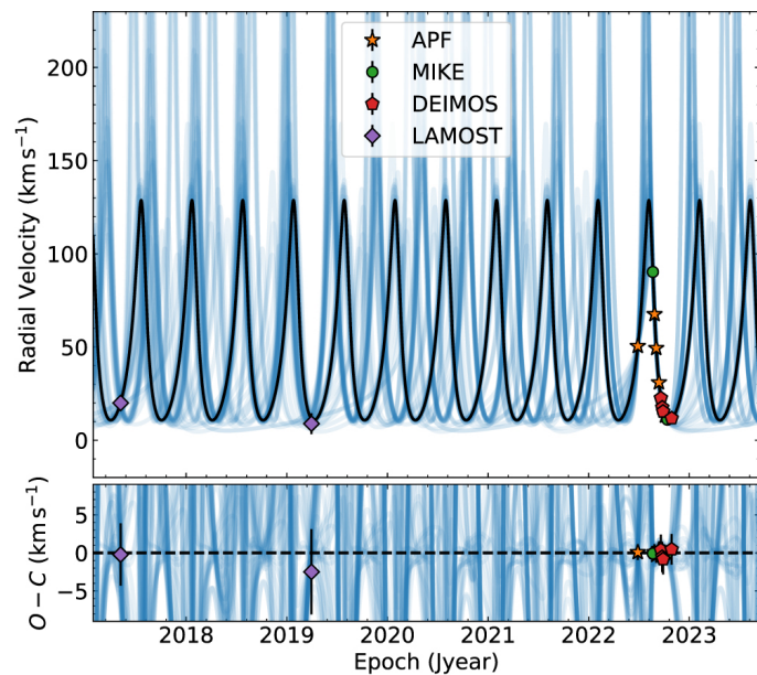
Figure 9. from Sukanya Chakrabarti et al 2023 Astron. J. 166 doi:10.3847/1538-3881/accf21 https://dx.doi.org/10.3847/1538-3881/accf21 © 2023. The Author(s). Published by the American Astronomical Society.
