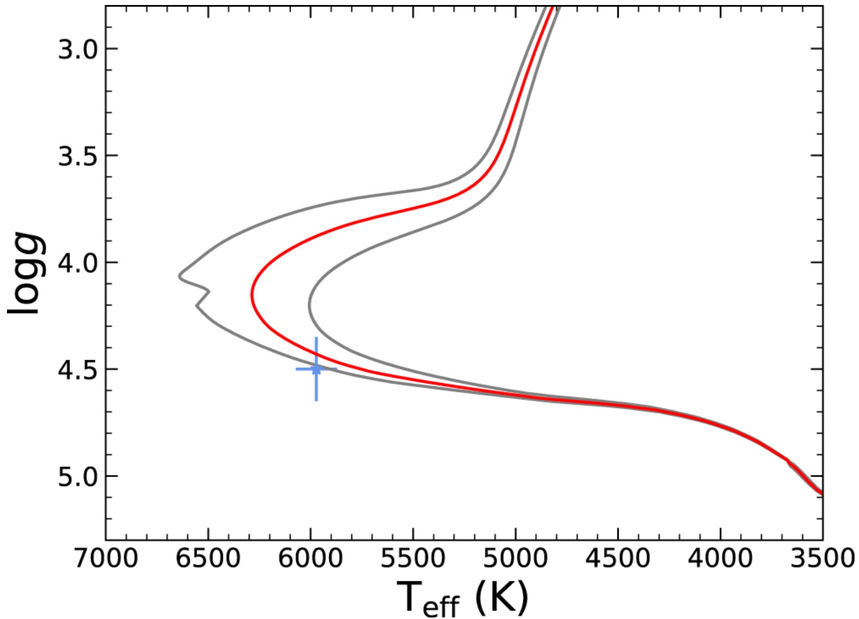
Figure 7. from Sukanya Chakrabarti et al 2023 Astron. J. 166 doi:10.3847/1538-3881/accf21 https://dx.doi.org/10.3847/1538-3881/accf21 © 2023. The Author(s). Published by the American Astronomical Society.
