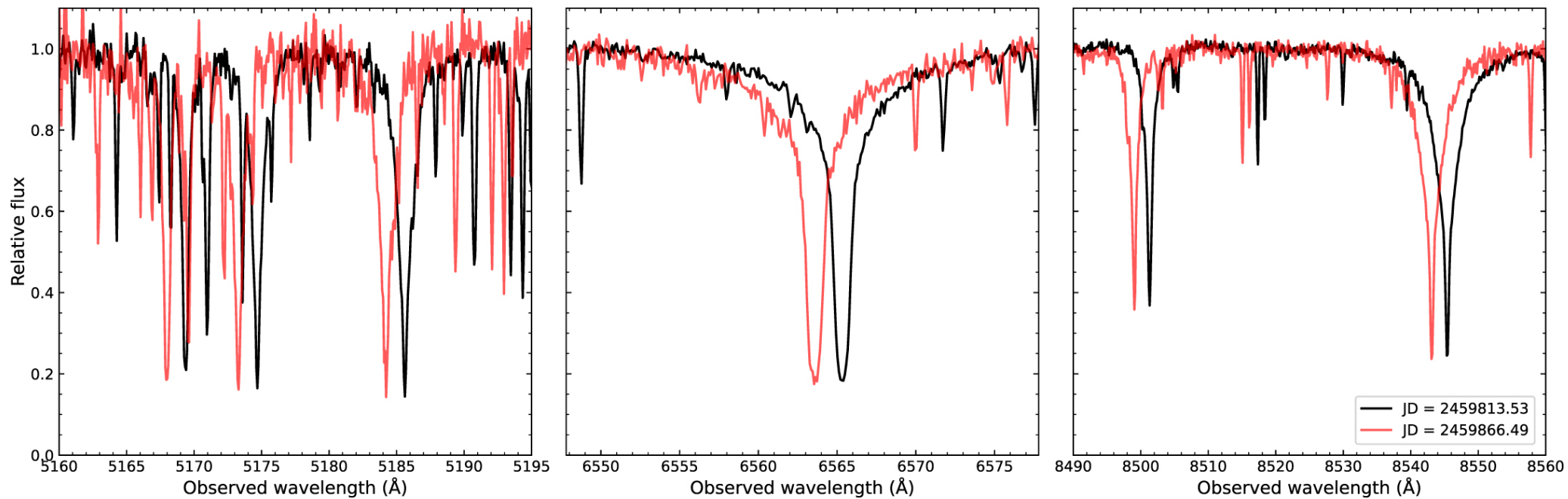
Figure 4. from Sukanya Chakrabarti et al 2023 Astron. J. 166 doi:10.3847/1538-3881/accf21 https://dx.doi.org/10.3847/1538-3881/accf21 © 2023. The Author(s). Published by the American Astronomical Society.
