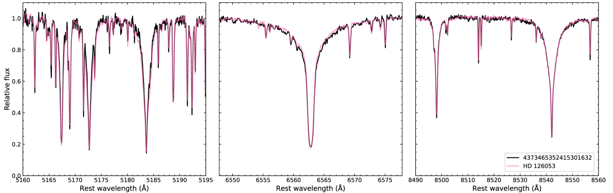
Figure 3. from Sukanya Chakrabarti et al 2023 Astron. J. 166 doi:10.3847/1538-3881/accf21 https://dx.doi.org/10.3847/1538-3881/accf21 © 2023. The Author(s). Published by the American Astronomical Society.
