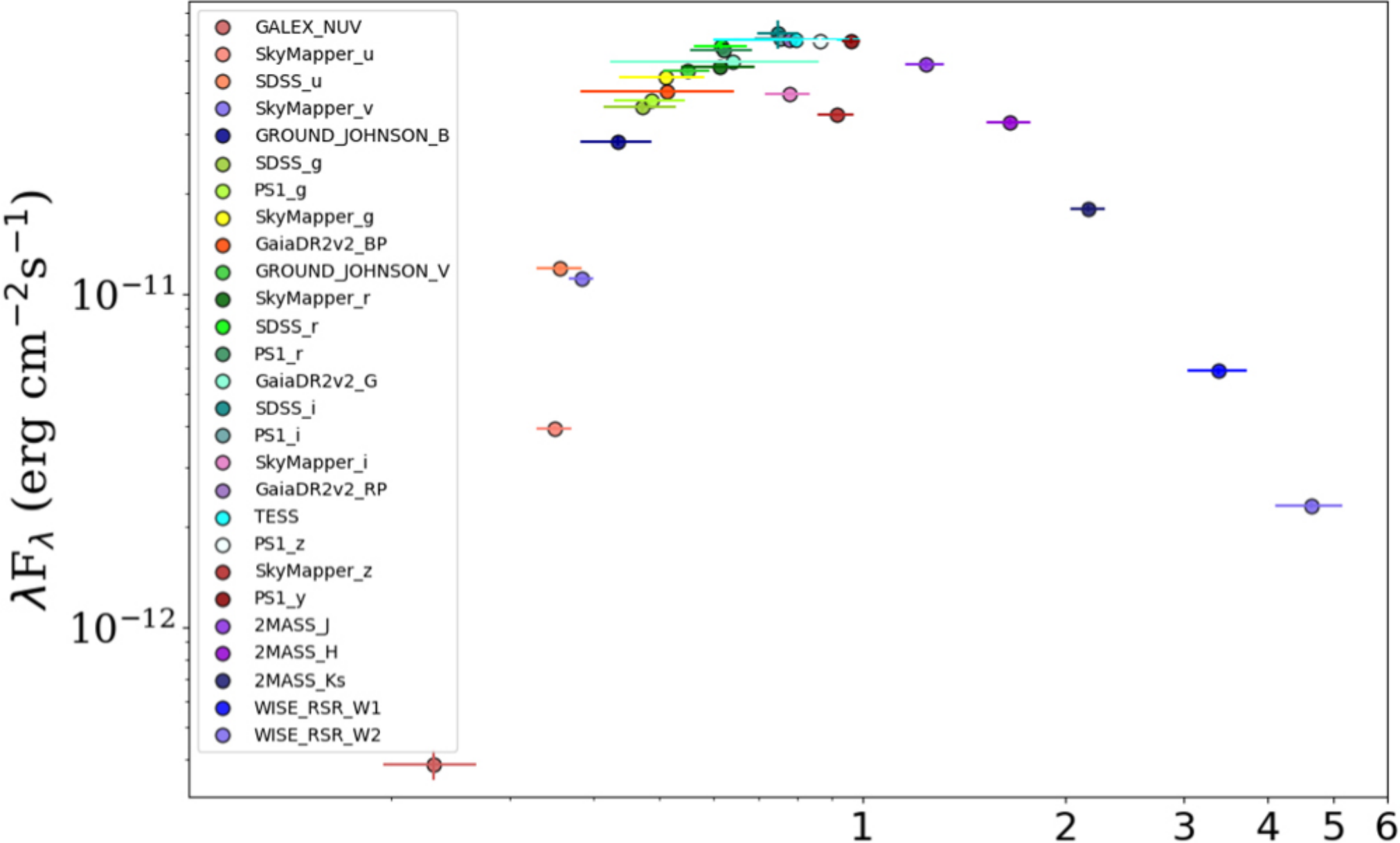
Figure 2. from Sukanya Chakrabarti et al 2023 Astron. J. 166 doi:10.3847/1538-3881/accf21 https://dx.doi.org/10.3847/1538-3881/accf21 © 2023. The Author(s). Published by the American Astronomical Society.
