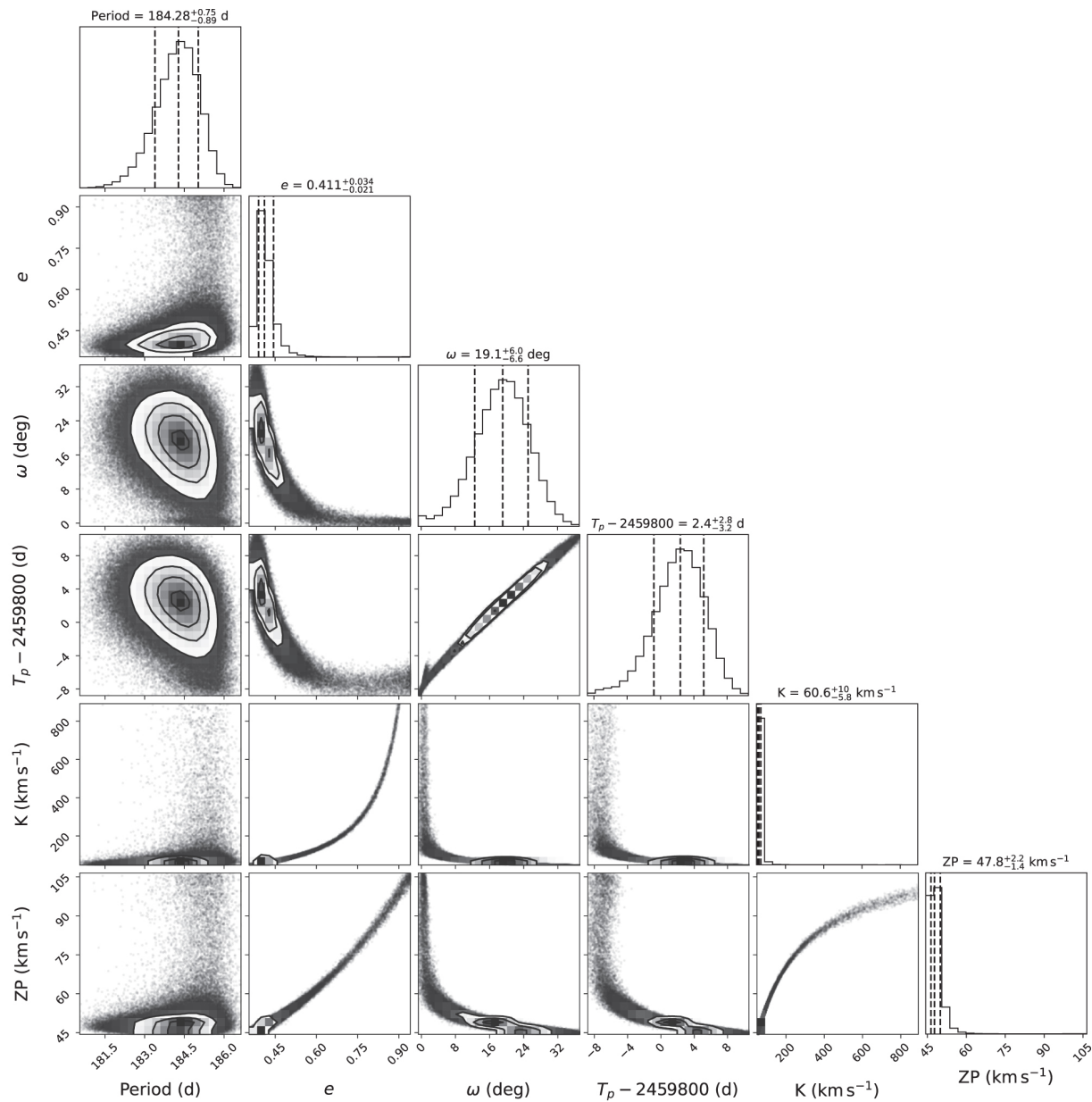
Figure 10. from Sukanya Chakrabarti et al 2023 Astron. J. 166 doi:10.3847/1538-3881/accf21 https://dx.doi.org/10.3847/1538-3881/accf21 © 2023. The Author(s). Published by the American Astronomical Society.
