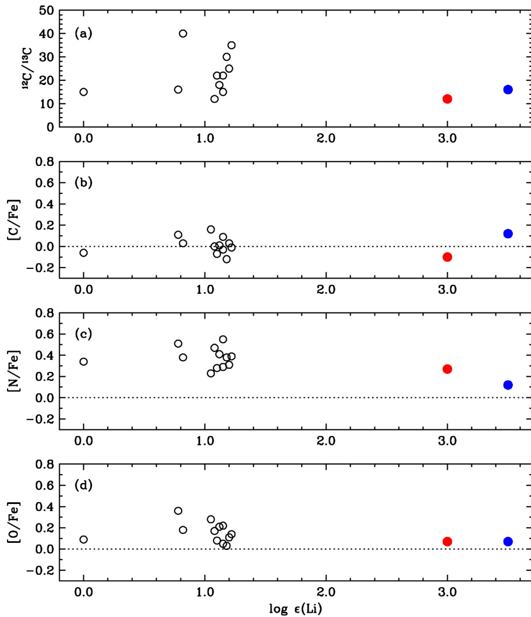
Figure 6. from Neel Nagarajan et al 2023 Astron. J. 165 doi:10.3847/1538-3881/acddda https://dx.doi.org/10.3847/1538-3881/acddda © 2023. The Author(s). Published by the American Astronomical Society.
