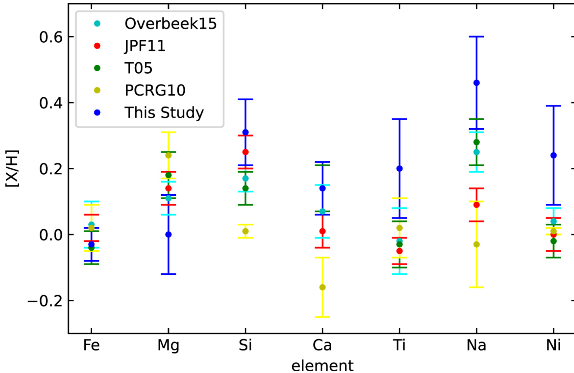
Figure 3. from Neel Nagarajan et al 2023 Astron. J. 165 doi:10.3847/1538-3881/acddda https://dx.doi.org/10.3847/1538-3881/acddda © 2023. The Author(s). Published by the American Astronomical Society.
