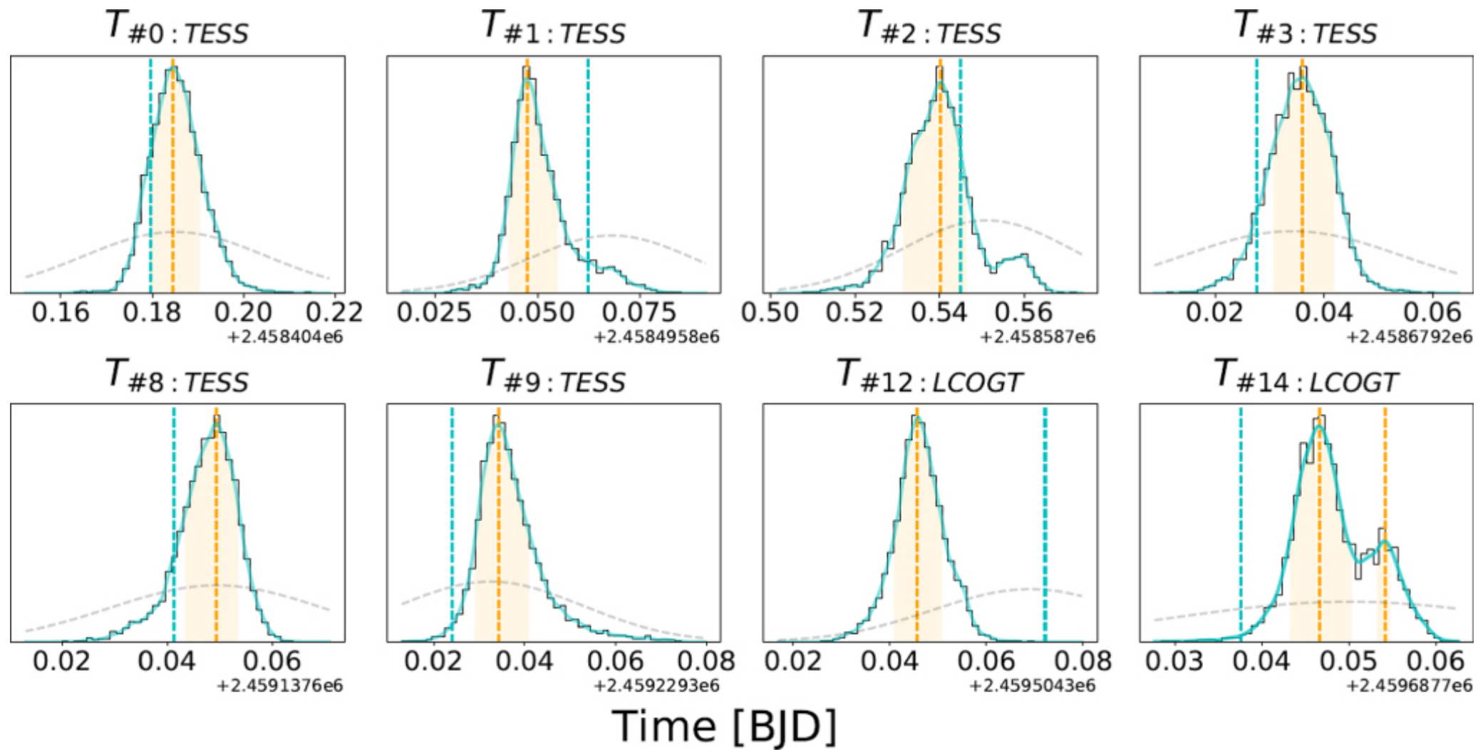
Figure 6. from Christopher Mann et al 2023 Astron. J. 165 doi:10.3847/1538-3881/acc8d4 https://dx.doi.org/10.3847/1538-3881/acc8d4 © 2023. The Author(s). Published by the American Astronomical Society.
