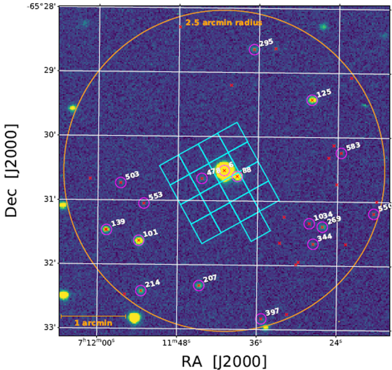
Figure 2. from Christopher Mann et al 2023 Astron. J. 165 doi:10.3847/1538-3881/acc8d4 https://dx.doi.org/10.3847/1538-3881/acc8d4 © 2023. The Author(s). Published by the American Astronomical Society.
