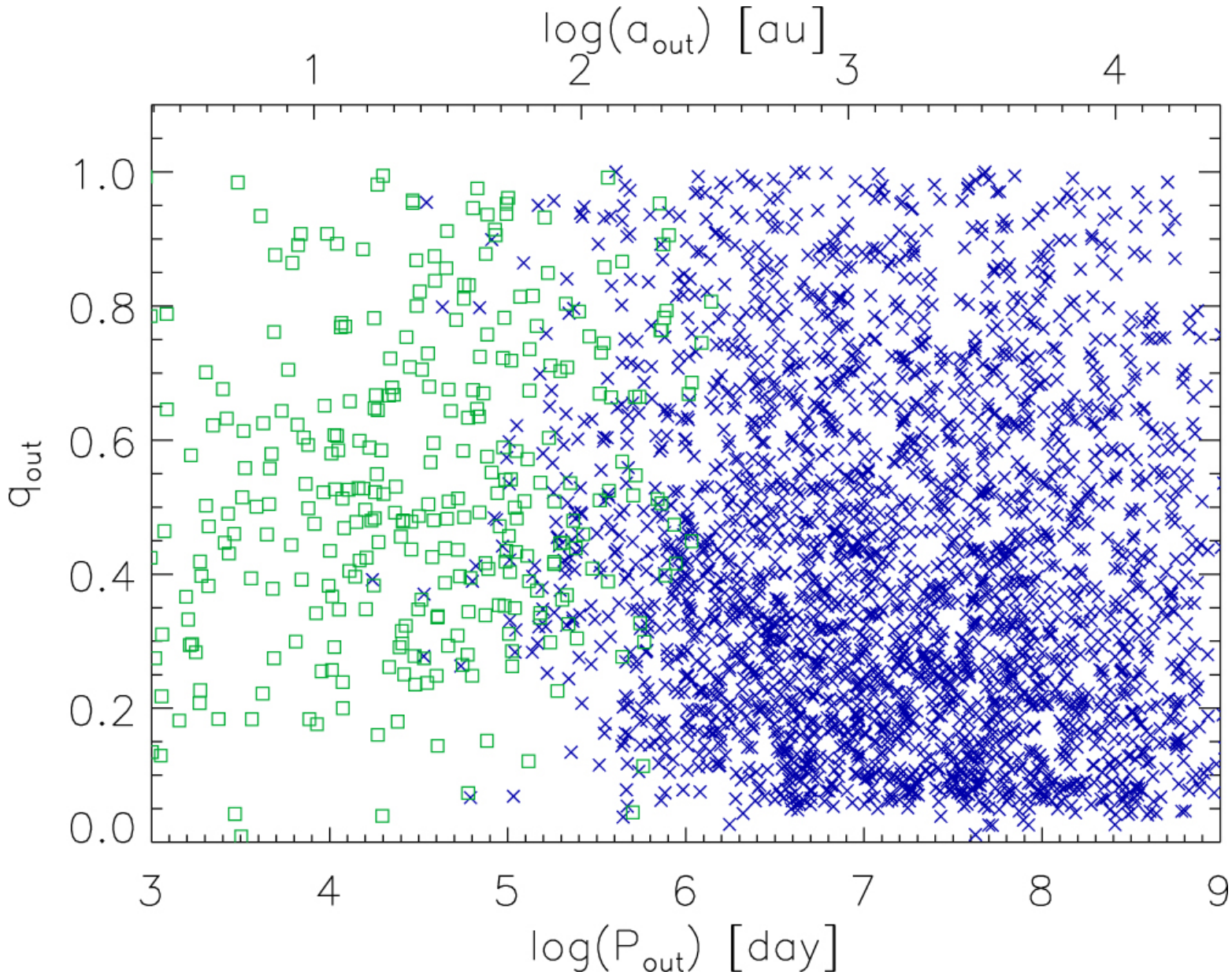
Figure 9. from Andrei Tokovinin 2023 Astron. J. 165 doi:10.3847/1538-3881/acc464 https://dx.doi.org/10.3847/1538-3881/acc464 © 2023. The Author(s). Published by the American Astronomical Society.
