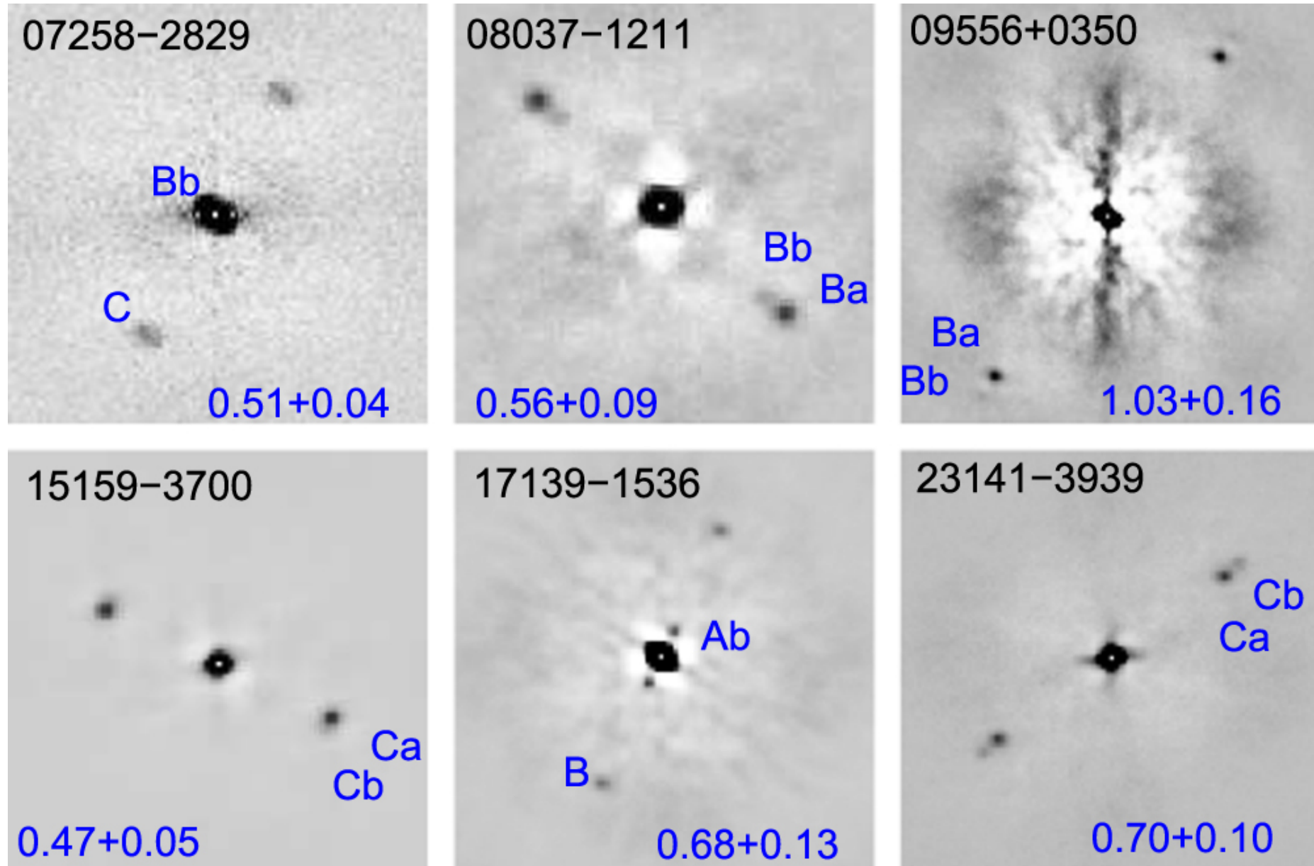
Figure 5. from Andrei Tokovinin 2023 Astron. J. 165 doi:10.3847/1538-3881/acc464 https://dx.doi.org/10.3847/1538-3881/acc464 © 2023. The Author(s). Published by the American Astronomical Society.
