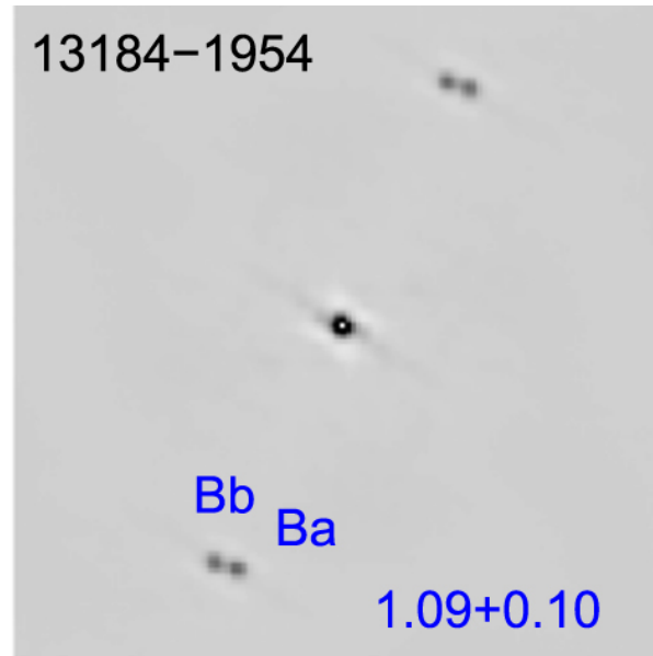
Figure 4. from Andrei Tokovinin 2023 Astron. J. 165 doi:10.3847/1538-3881/acc464 https://dx.doi.org/10.3847/1538-3881/acc464 © 2023. The Author(s). Published by the American Astronomical Society.
