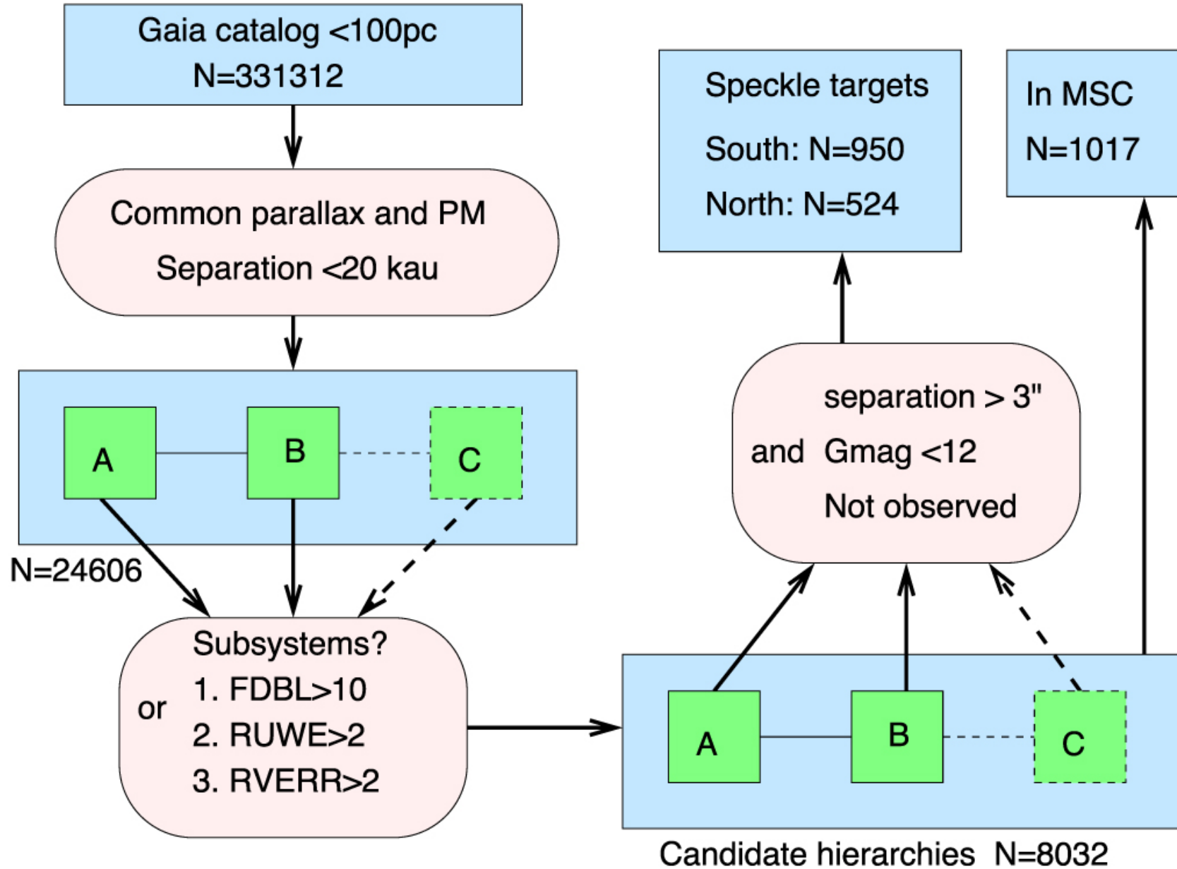
Figure 3. from Andrei Tokovinin 2023 Astron. J. 165 doi:10.3847/1538-3881/acc464 https://dx.doi.org/10.3847/1538-3881/acc464 © 2023. The Author(s). Published by the American Astronomical Society.
