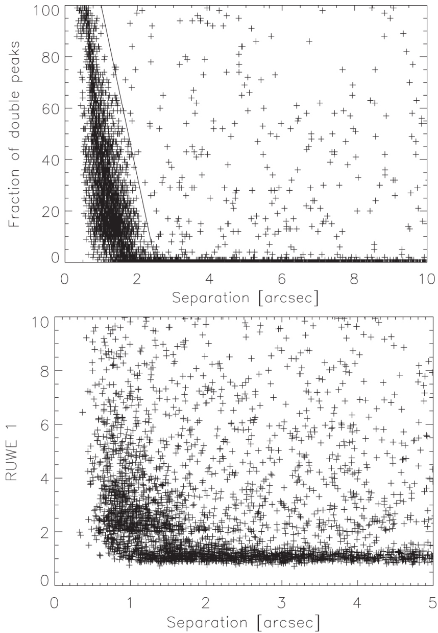
Figure 2. from Andrei Tokovinin 2023 Astron. J. 165 doi:10.3847/1538-3881/acc464 https://dx.doi.org/10.3847/1538-3881/acc464 © 2023. The Author(s). Published by the American Astronomical Society.
