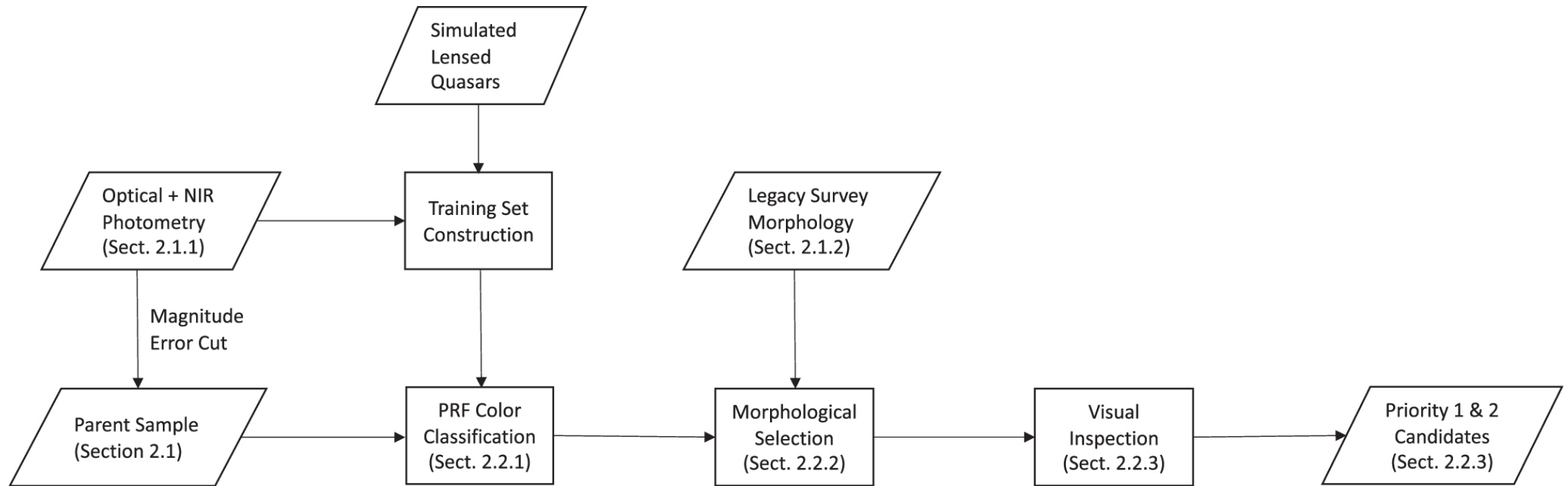
Figure 1. from Minghao Yue et al 2023 Astron. J. 165 doi:10.3847/1538-3881/acc2be https://dx.doi.org/10.3847/1538-3881/acc2be © 2023. The Author(s). Published by the American Astronomical Society.
