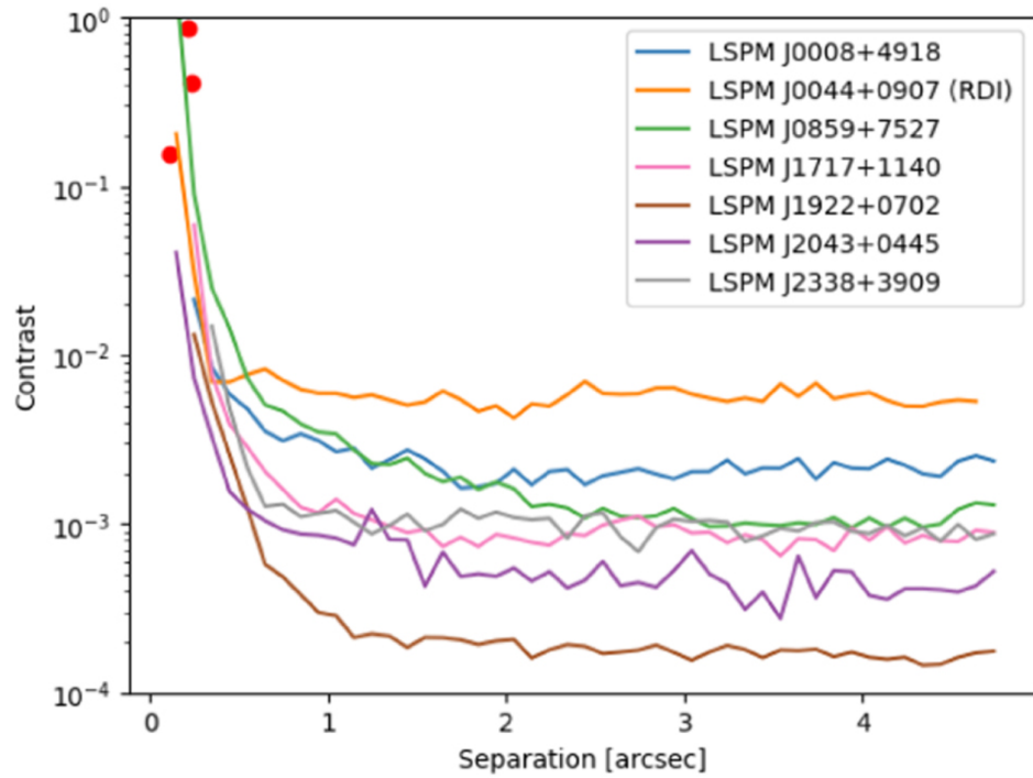
Figure 8. from Taichi Uyama et al 2023 Astron. J. 165 doi:10.3847/1538-3881/acbf37 https://dx.doi.org/10.3847/1538-3881/acbf37 © 2023. The Author(s). Published by the American Astronomical Society.
