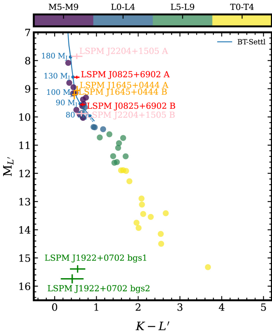
Figure 6. from Taichi Uyama et al 2023 Astron. J. 165 doi:10.3847/1538-3881/acbf37 https://dx.doi.org/10.3847/1538-3881/acbf37 © 2023. The Author(s). Published by the American Astronomical Society.
