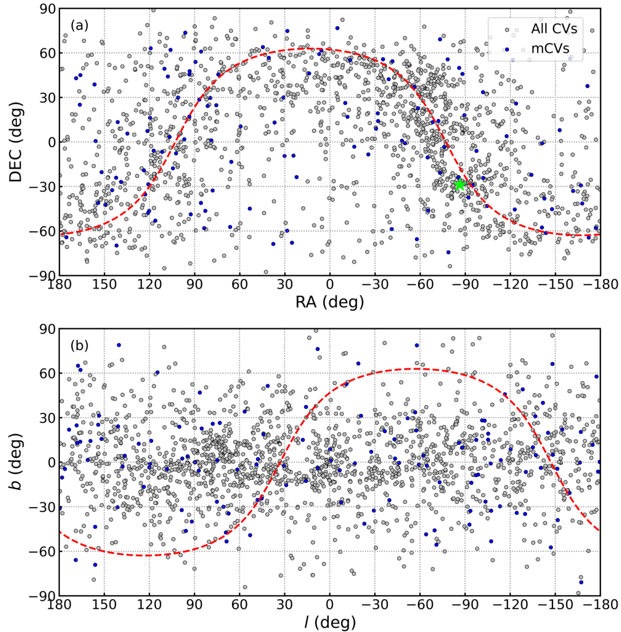
Figure 6. from Remziye Canbay et al 2023 Astron. J. 165 doi:10.3847/1538-3881/acbead https://dx.doi.org/10.3847/1538-3881/acbead © 2023. The Author(s). Published by the American Astronomical Society.
