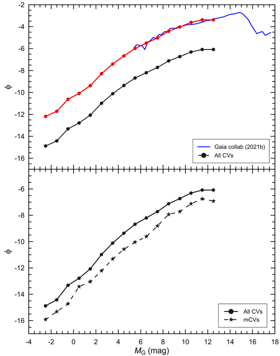
Figure 12. from Remziye Canbay et al 2023 Astron. J. 165 doi:10.3847/1538-3881/acbead https://dx.doi.org/10.3847/1538-3881/acbead © 2023. The Author(s). Published by the American Astronomical Society.
