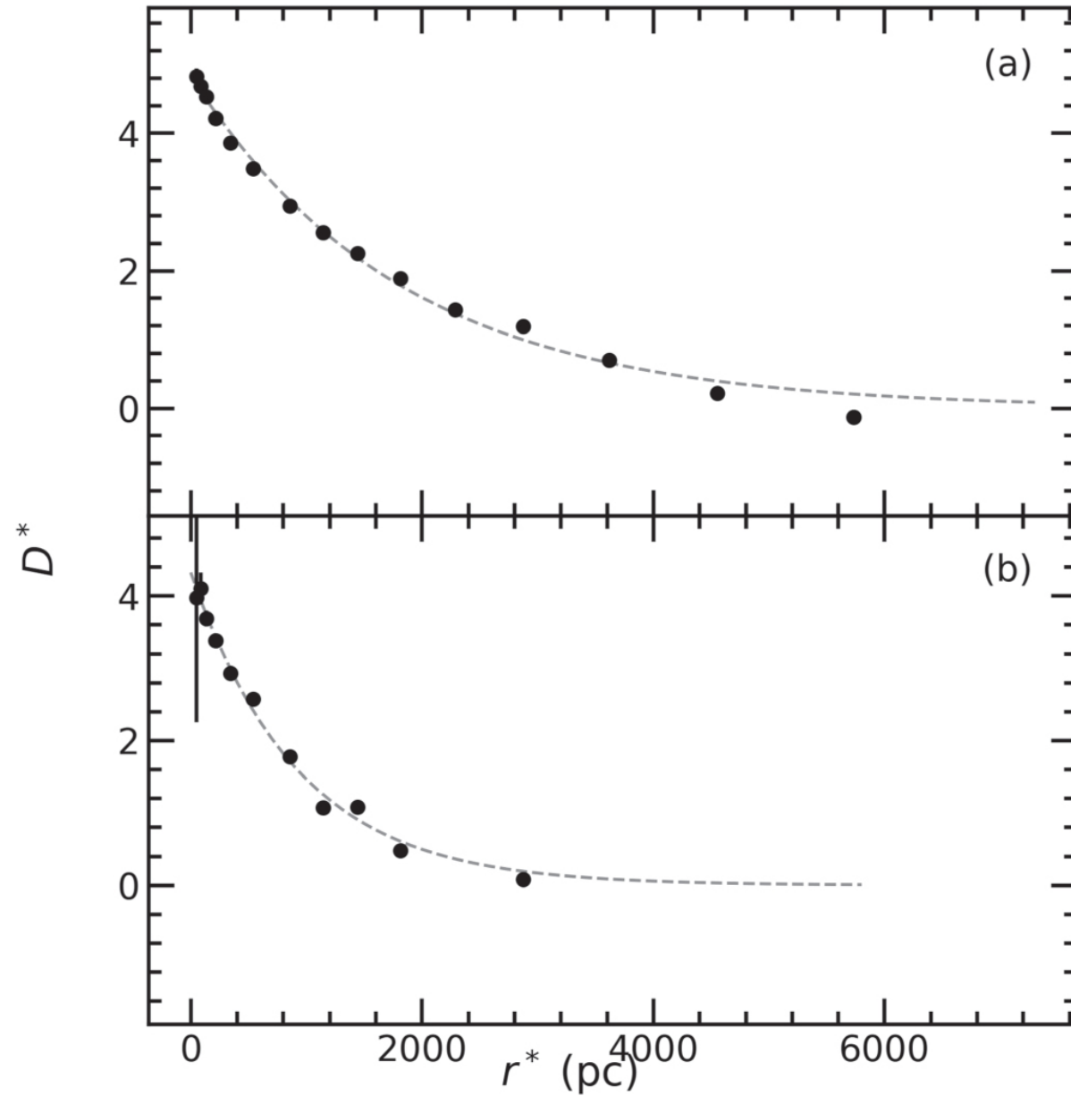
Figure 11. from Remziye Canbay et al 2023 Astron. J. 165 doi:10.3847/1538-3881/acbead https://dx.doi.org/10.3847/1538-3881/acbead © 2023. The Author(s). Published by the American Astronomical Society.
