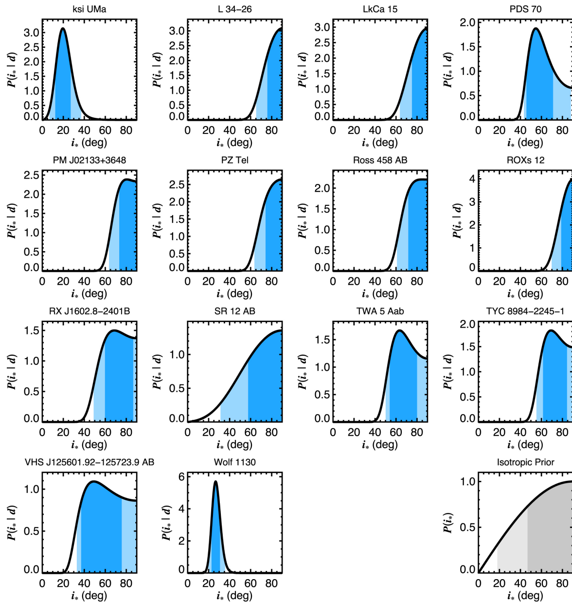
Figure 8. from Brendan P. Bowler et al 2023 Astron. J. 165 doi:10.3847/1538-3881/acbd34 https://dx.doi.org/10.3847/1538-3881/acbd34 © 2023. The Author(s). Published by the American Astronomical Society.
