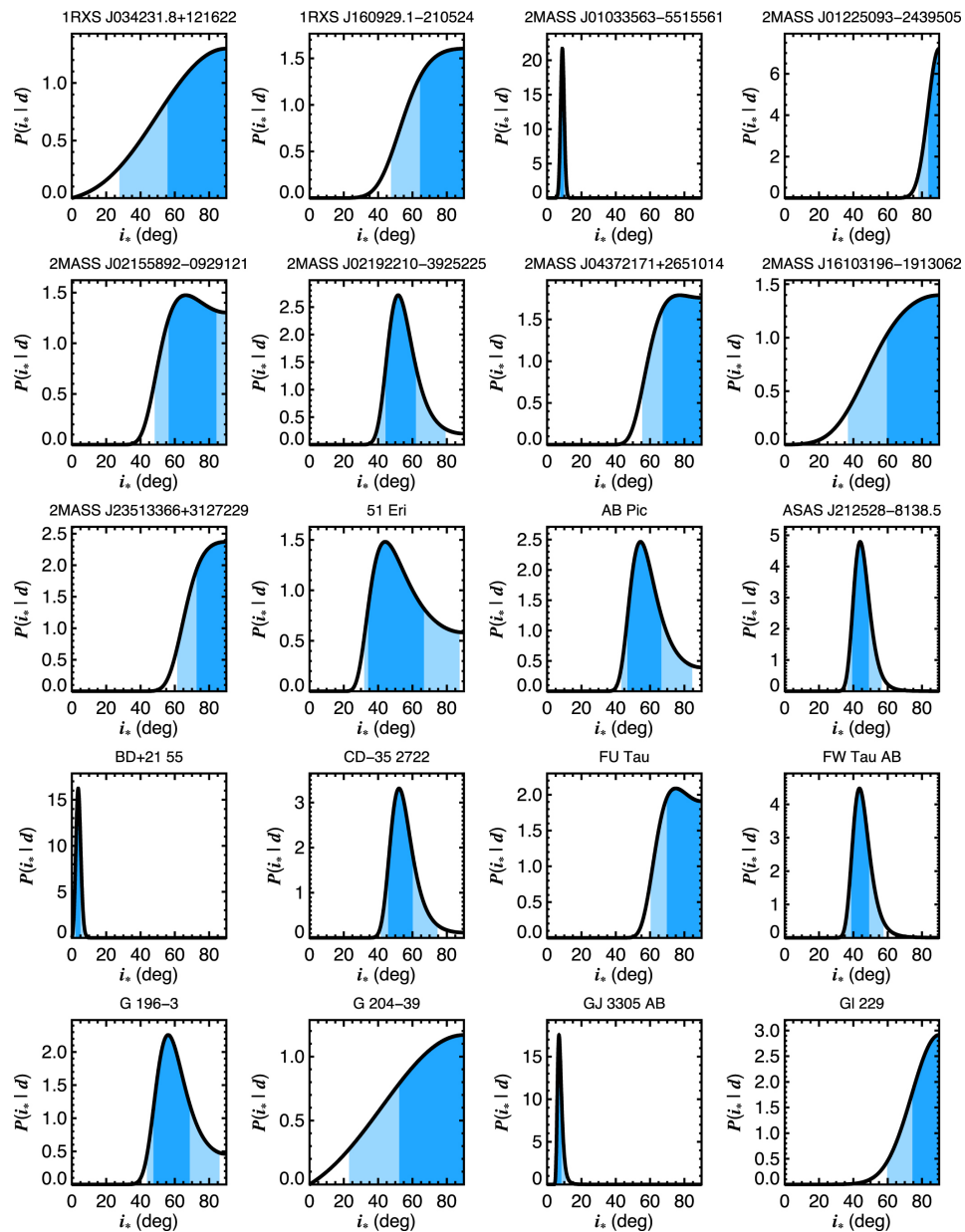
Figure 6. from Brendan P. Bowler et al 2023 Astron. J. 165 doi:10.3847/1538-3881/acbd34 https://dx.doi.org/10.3847/1538-3881/acbd34 © 2023. The Author(s). Published by the American Astronomical Society.
