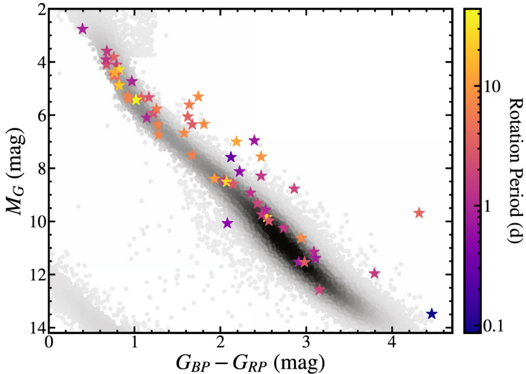
Figure 3. from Brendan P. Bowler et al 2023 Astron. J. 165 doi:10.3847/1538-3881/acbd34 https://dx.doi.org/10.3847/1538-3881/acbd34 © 2023. The Author(s). Published by the American Astronomical Society.
