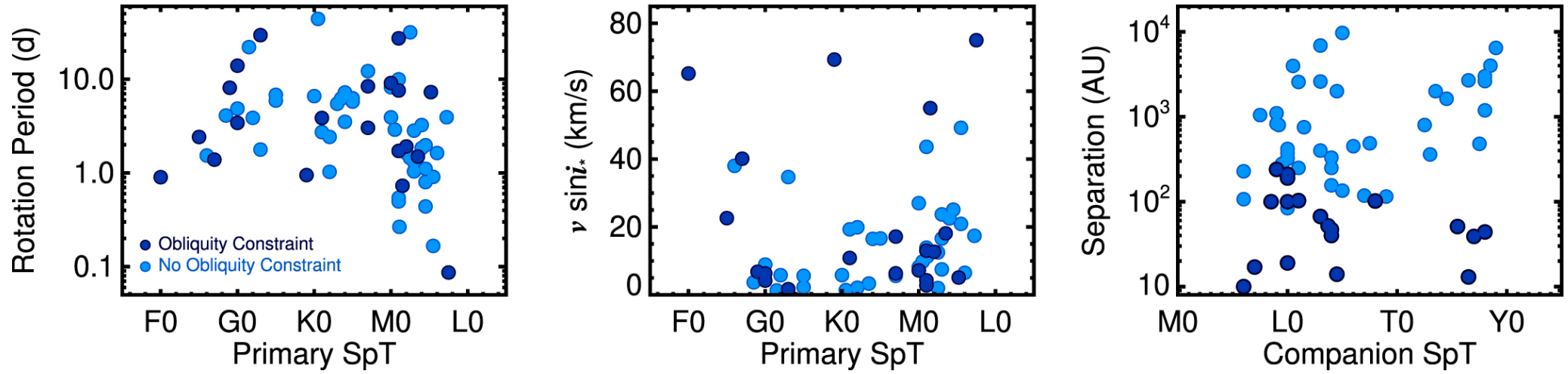
Figure 2. from Brendan P. Bowler et al 2023 Astron. J. 165 doi:10.3847/1538-3881/acbd34 https://dx.doi.org/10.3847/1538-3881/acbd34 © 2023. The Author(s). Published by the American Astronomical Society.
