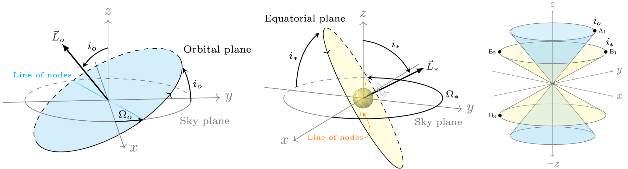
Figure 1. from Brendan P. Bowler et al 2023 Astron. J. 165 doi:10.3847/1538-3881/acbd34 https://dx.doi.org/10.3847/1538-3881/acbd34 © 2023. The Author(s). Published by the American Astronomical Society.
