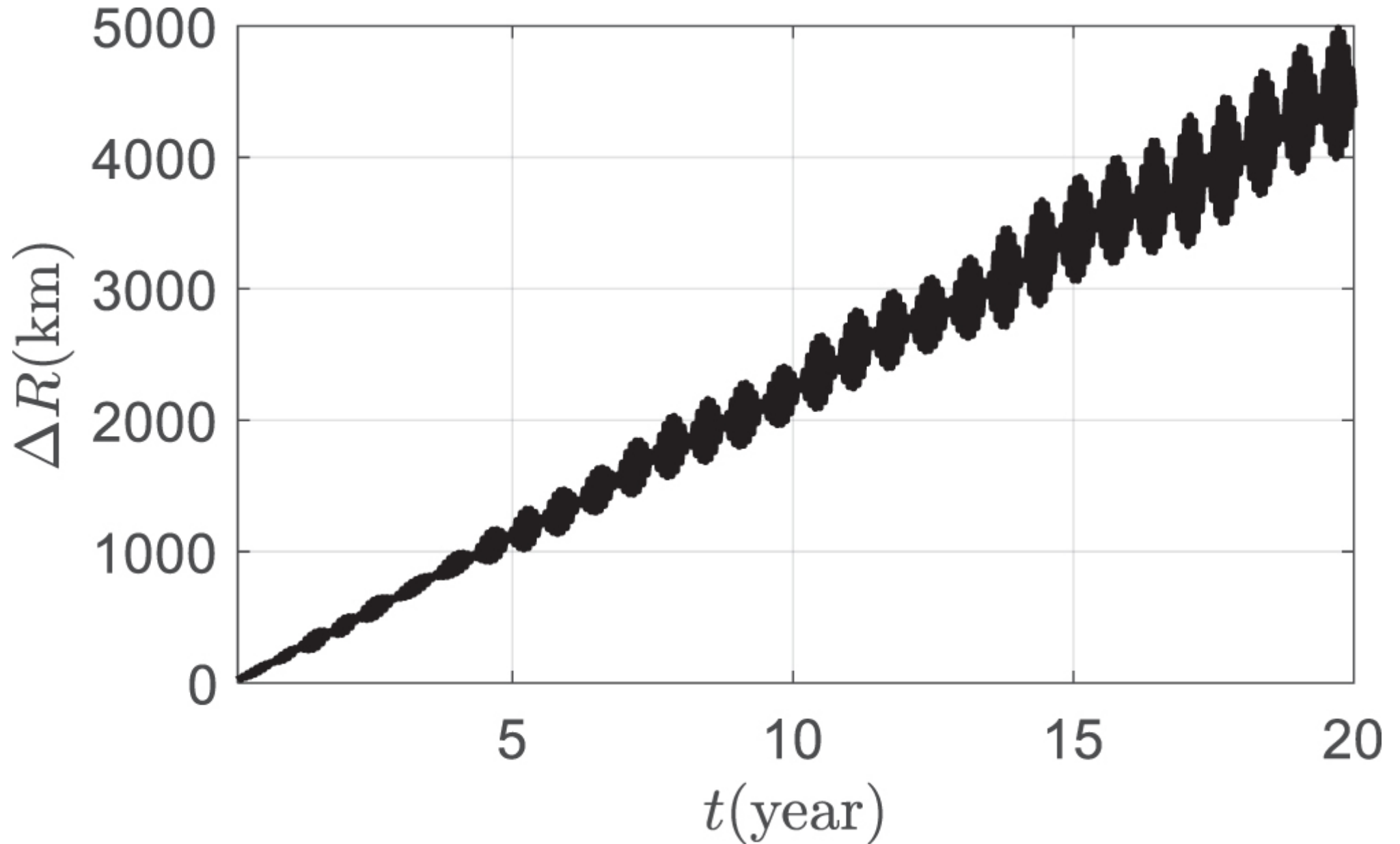
Figure 4. from Bo-Sheng Li and Xi-Yun Hou 2023 Astron. J. 165 doi:10.3847/1538-3881/acbafa https://dx.doi.org/10.3847/1538-3881/acbafa © 2023. The Author(s). Published by the American Astronomical Society.
