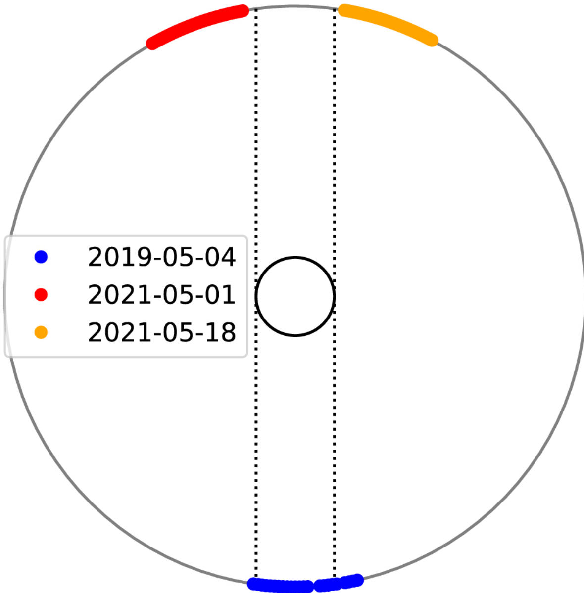
Figure 1. from Marshall C. Johnson et al 2023 Astron. J. 165 doi:10.3847/1538-3881/acb7e2 https://dx.doi.org/10.3847/1538-3881/acb7e2 © 2023. The Author(s). Published by the American Astronomical Society.
