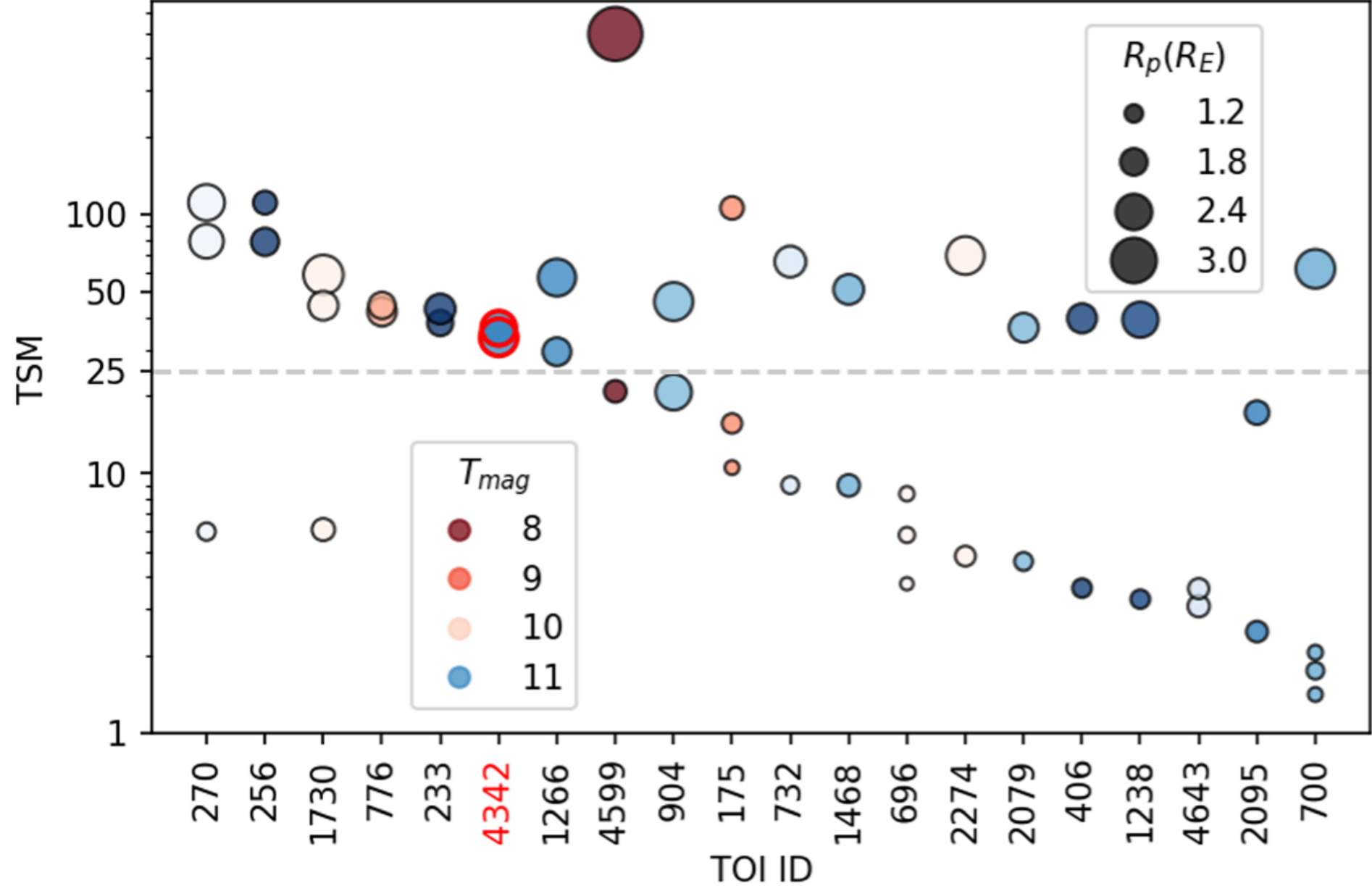
Figure 7. from Evan Tey et al 2023 Astron. J. 165 doi:10.3847/1538-3881/acaf88 https://dx.doi.org/10.3847/1538-3881/acaf88 © 2023. The Author(s). Published by the American Astronomical Society.
