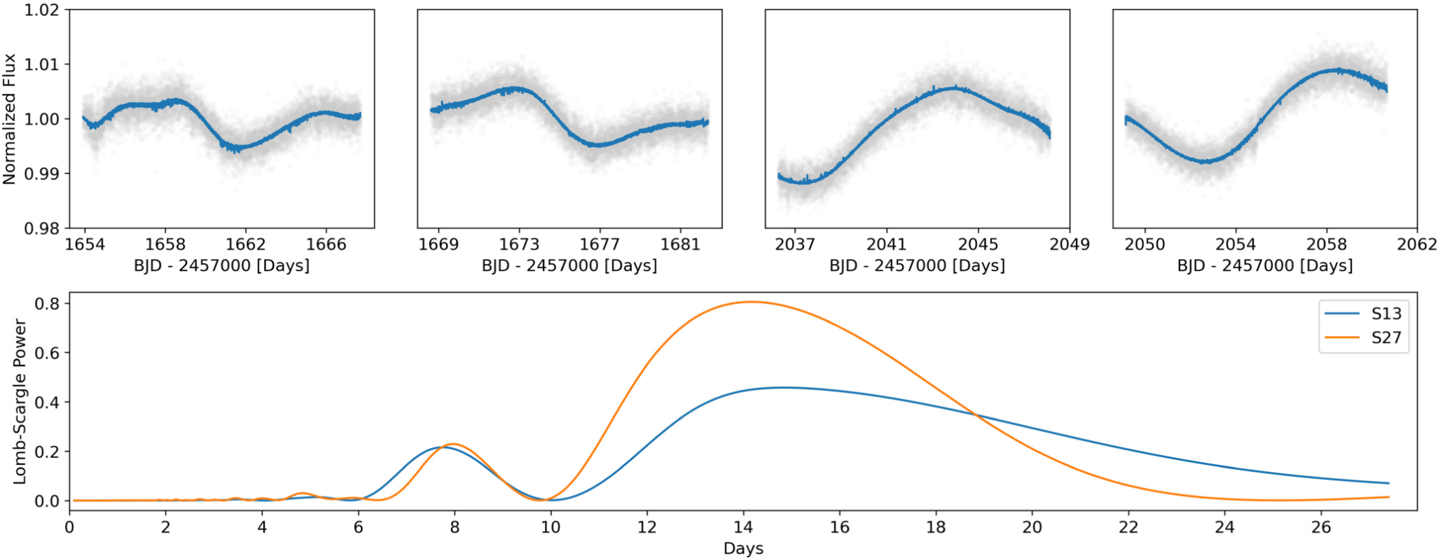
Figure 2. from Evan Tey et al 2023 Astron. J. 165 doi:10.3847/1538-3881/acaf88 https://dx.doi.org/10.3847/1538-3881/acaf88 © 2023. The Author(s). Published by the American Astronomical Society.
