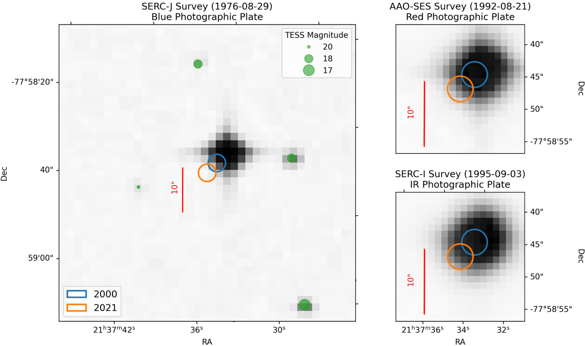
Figure 1. from Evan Tey et al 2023 Astron. J. 165 doi:10.3847/1538-3881/acaf88 https://dx.doi.org/10.3847/1538-3881/acaf88 © 2023. The Author(s). Published by the American Astronomical Society.
