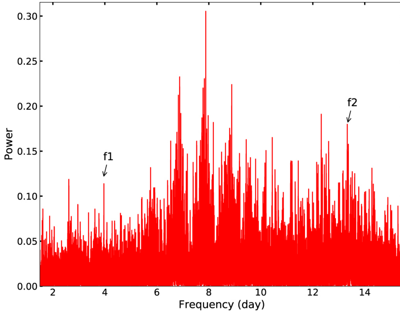
Figure 9. from Jaynand Maurya et al 2023 Astron. J. 165 doi:10.3847/1538-3881/acad7e https://dx.doi.org/10.3847/1538-3881/acad7e © 2023. The Author(s). Published by the American Astronomical Society.
