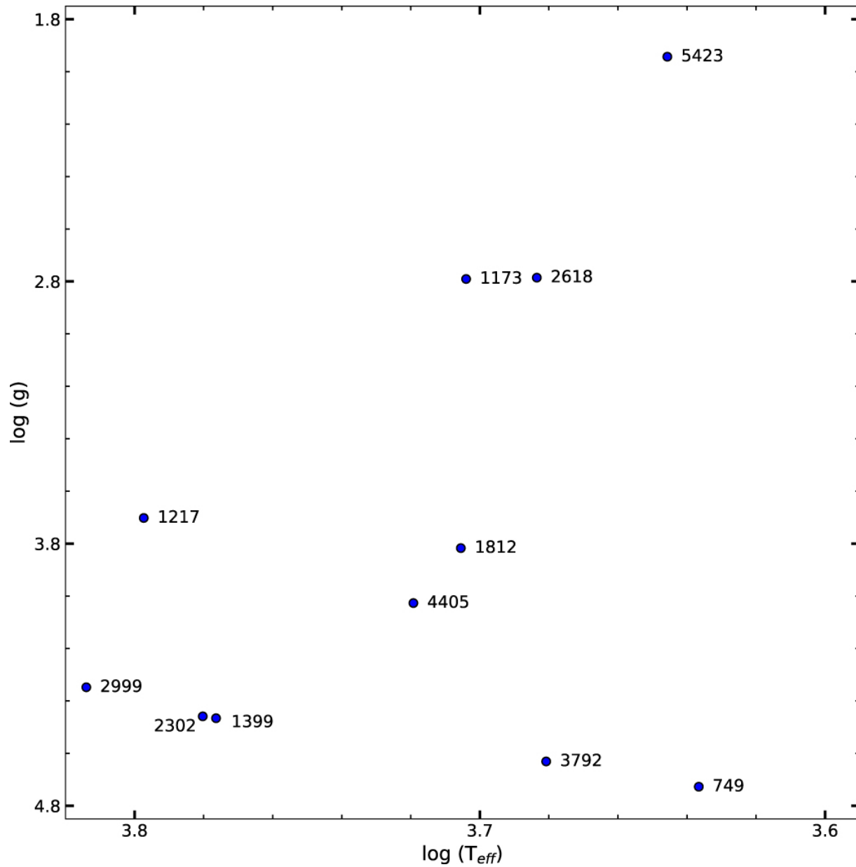
Figure 8. from Jayanand Maurya et al 2023 Astron. J. 165 doi:10.3847/1538-3881/acad7e https://dx.doi.org/10.3847/1538-3881/acad7e © 2023. The Author(s). Published by the American Astronomical Society.
