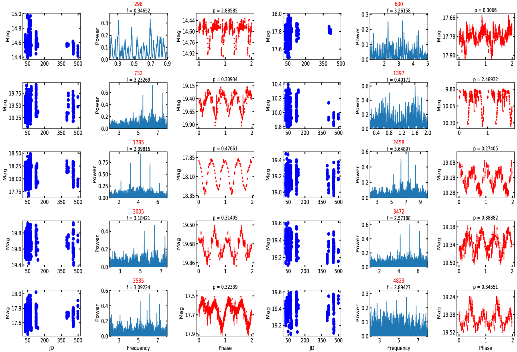
Figure 6. from Jayanand Maurya et al 2023 Astron. J. 165 doi:10.3847/1538-3881/acad7e https://dx.doi.org/10.3847/1538-3881/acad7e © 2023. The Author(s). Published by the American Astronomical Society.
