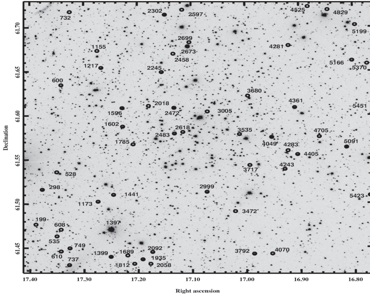
Figure 2. from Jayanand Maurya et al 2023 Astron. J. 165 doi:10.3847/1538-3881/acad7e https://dx.doi.org/10.3847/1538-3881/acad7e © 2023. The Author(s). Published by the American Astronomical Society.
