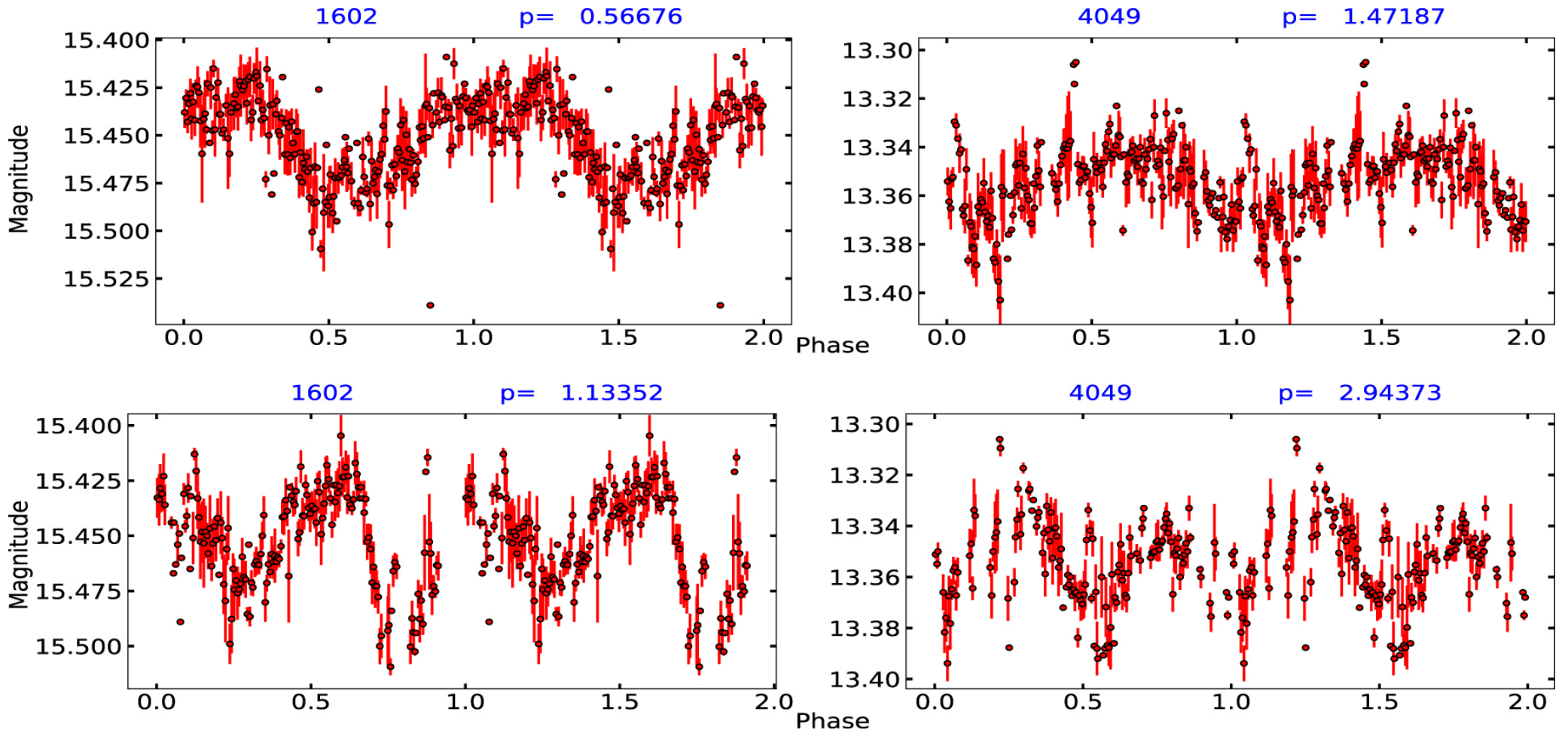
Figure 12. from Jayanand Maurya et al 2023 Astron. J. 165 doi:10.3847/1538-3881/acad7e https://dx.doi.org/10.3847/1538-3881/acad7e © 2023. The Author(s). Published by the American Astronomical Society.
