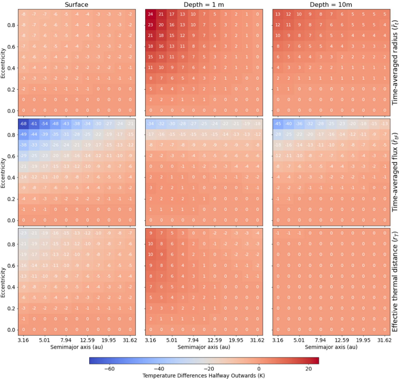
Figure 7. from Anastasios Gkotsinas et al 2023 Astron. J. 165 doi:10.3847/1538-3881/acaafd https://dx.doi.org/10.3847/1538-3881/acaafd © 2023. The Author(s). Published by the American Astronomical Society.
