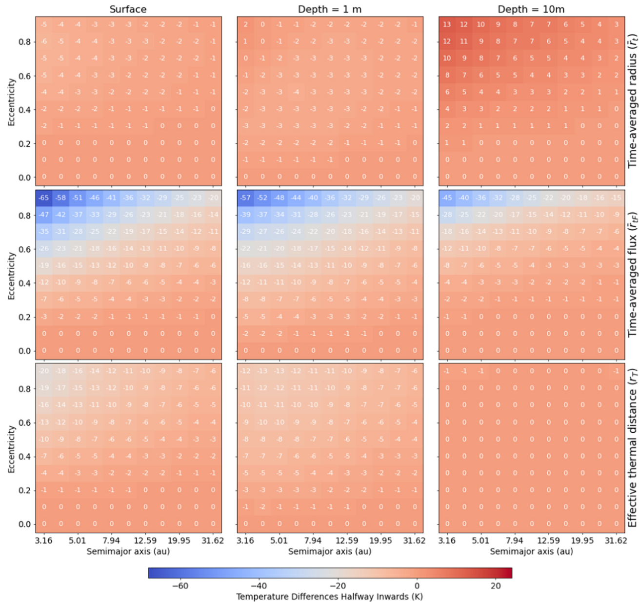
Figure 6. from Anastasios Gkotsinas et al 2023 Astron. J. 165 doi:10.3847/1538-3881/acaafd https://dx.doi.org/10.3847/1538-3881/acaafd © 2023. The Author(s). Published by the American Astronomical Society.
