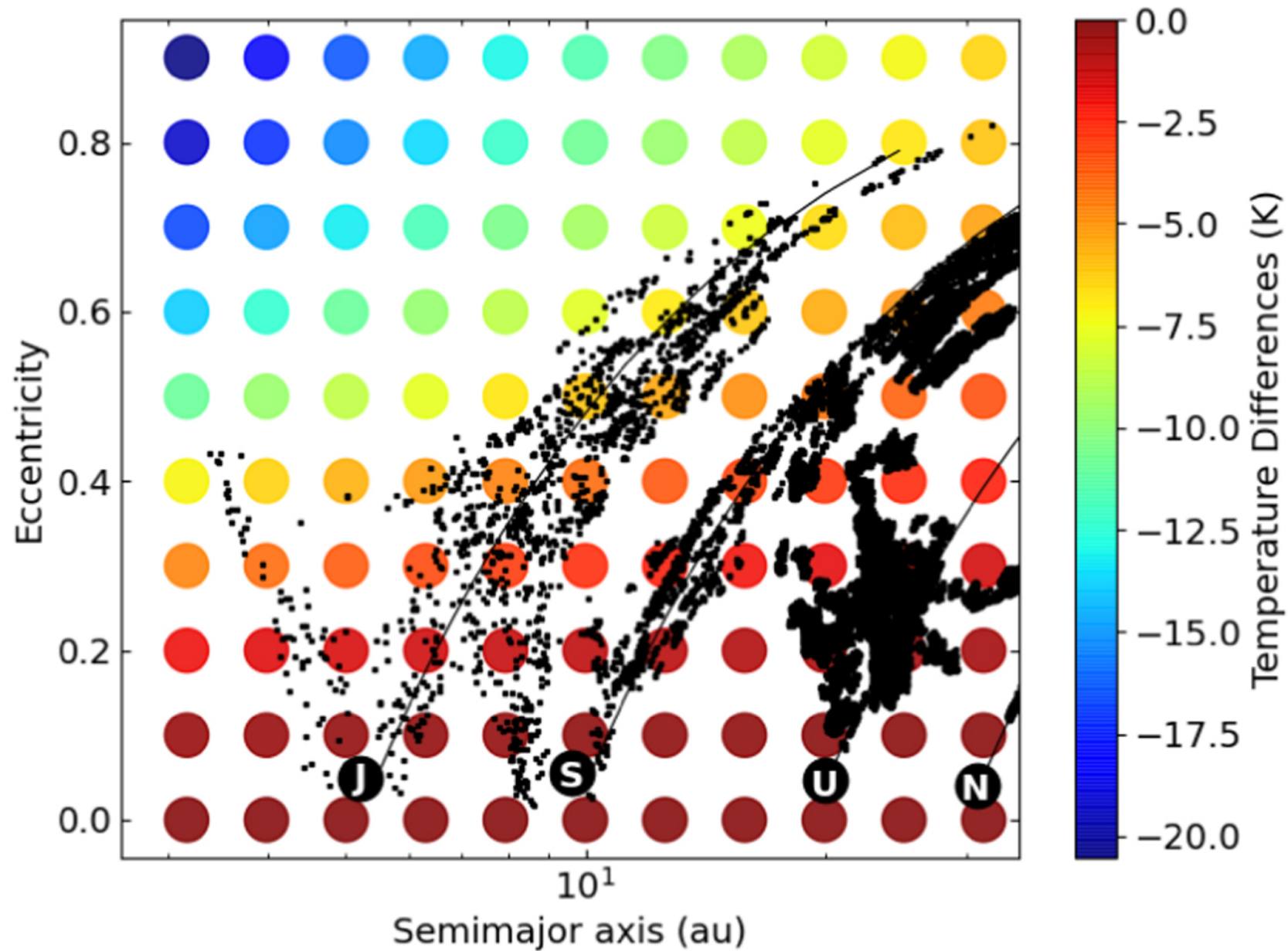
Figure 5. from Anastasios Gkotsinas et al 2023 Astron. J. 165 doi:10.3847/1538-3881/acaafd https://dx.doi.org/10.3847/1538-3881/acaafd © 2023. The Author(s). Published by the American Astronomical Society.
