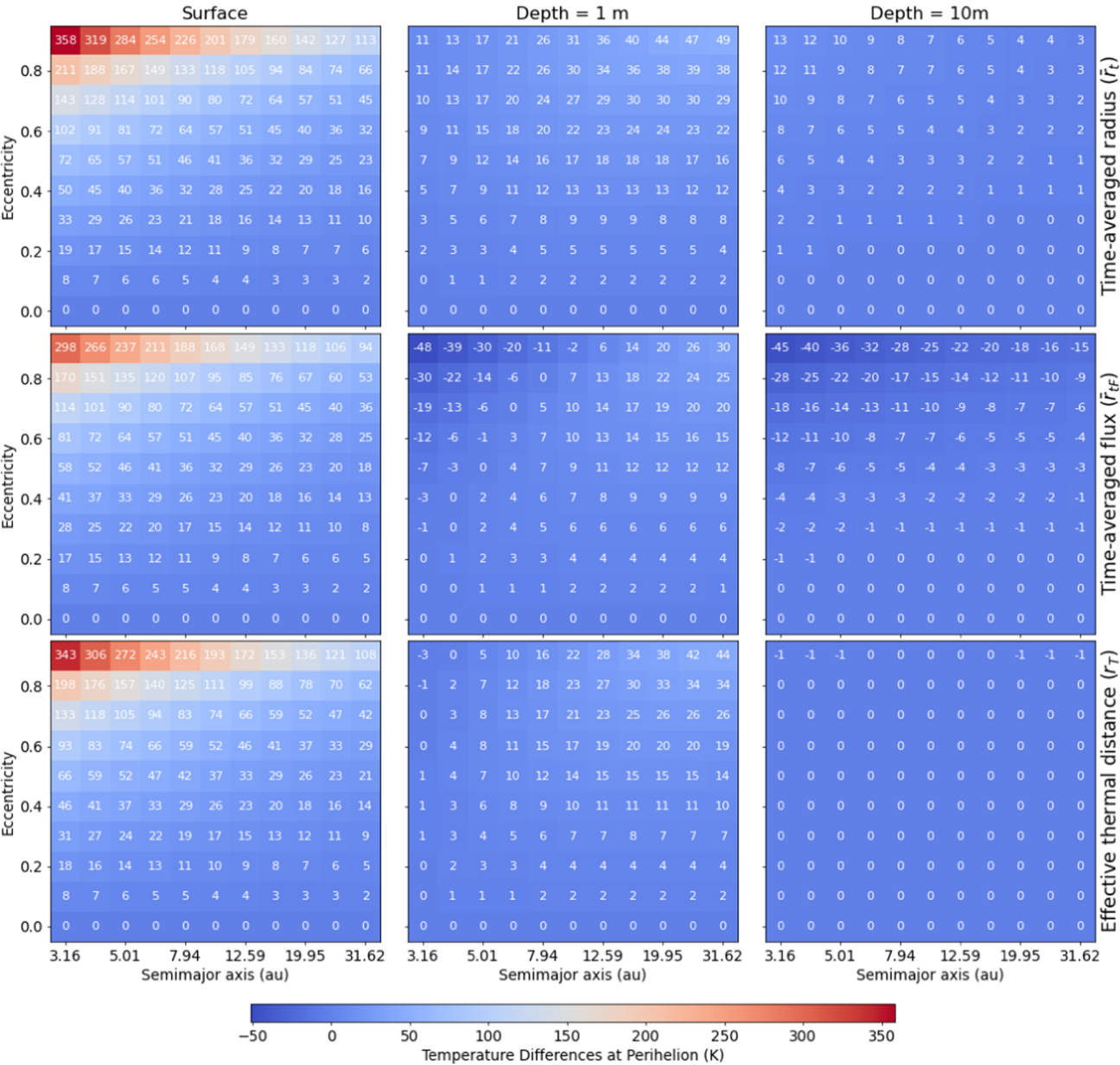
Figure 3. from Anastasios Gkotsinas et al 2023 Astron. J. 165 doi:10.3847/1538-3881/acaafd https://dx.doi.org/10.3847/1538-3881/acaafd © 2023. The Author(s). Published by the American Astronomical Society.
