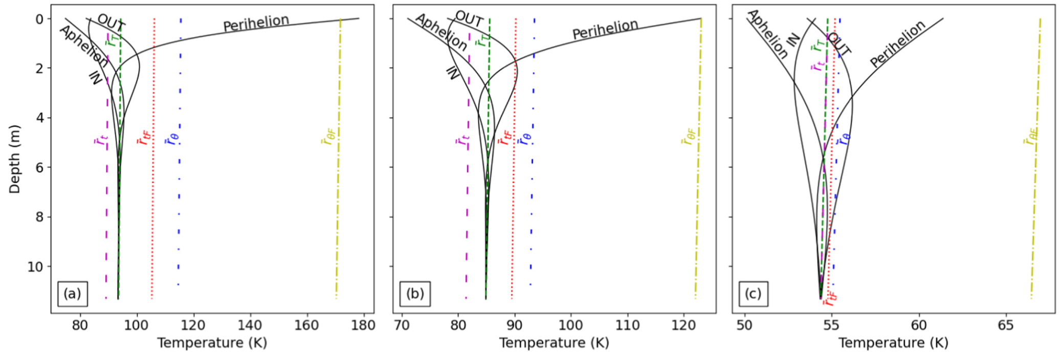
Figure 2. from Anastasios Gkotsinas et al 2023 Astron. J. 165 doi:10.3847/1538-3881/acaafd https://dx.doi.org/10.3847/1538-3881/acaafd © 2023. The Author(s). Published by the American Astronomical Society.
