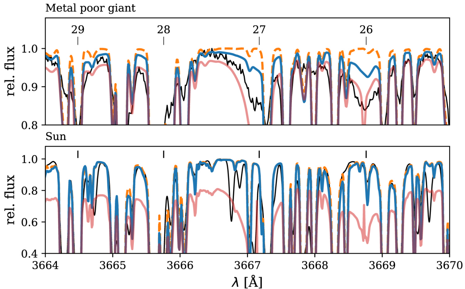
Figure 9. from Adam J. Wheeler et al 2023 Astron. J. 165 doi:10.3847/1538-3881/acaad https://dx.doi.org/10.3847/1538-3881/acaad © 2023. The Author(s). Published by the American Astronomical Society.
