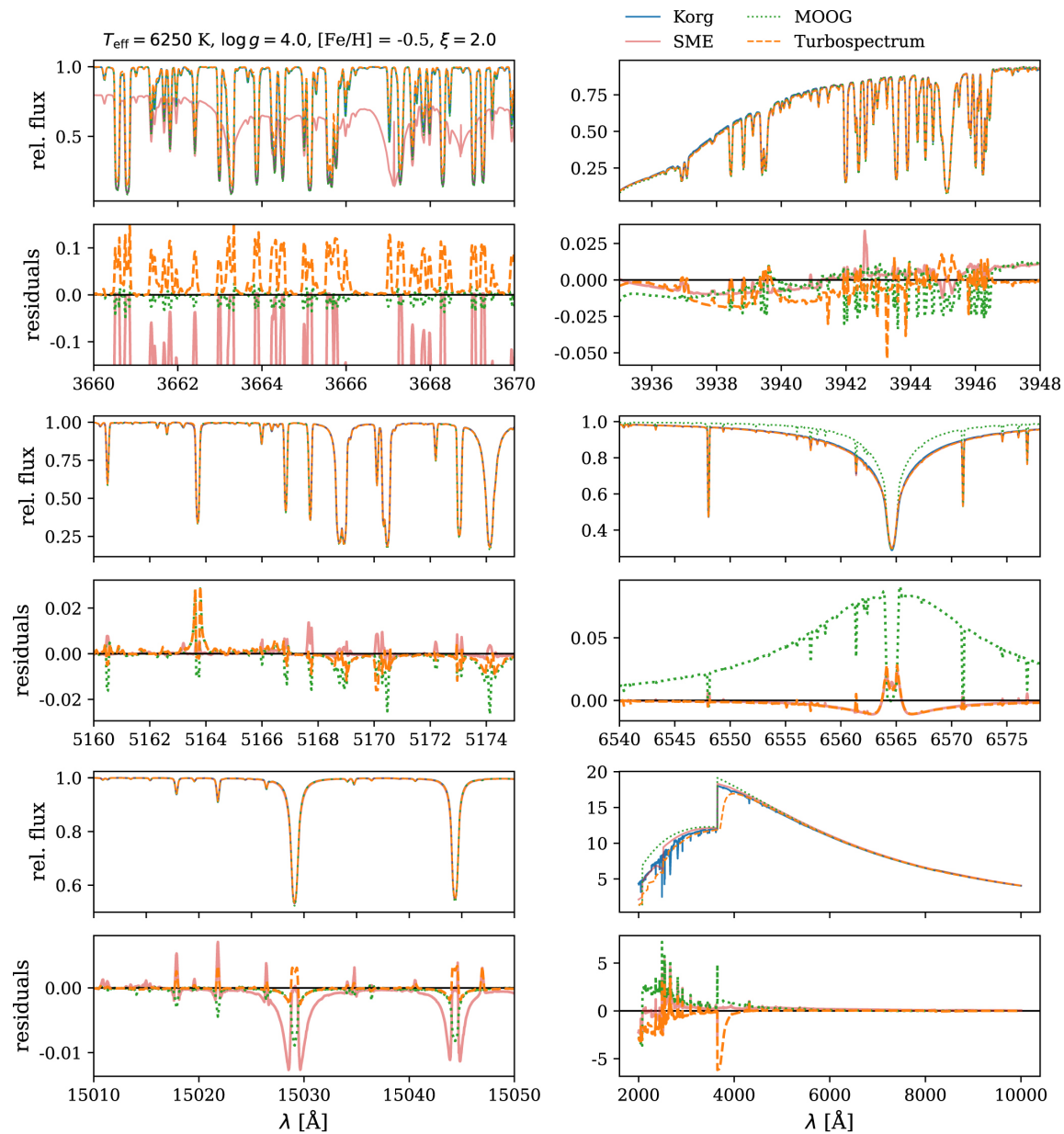
Figure 8. from Adam J. Wheeler et al 2023 Astron. J. 165 doi:10.3847/1538-3881/acaad https://dx.doi.org/10.3847/1538-3881/acaad © 2023. The Author(s). Published by the American Astronomical Society.
