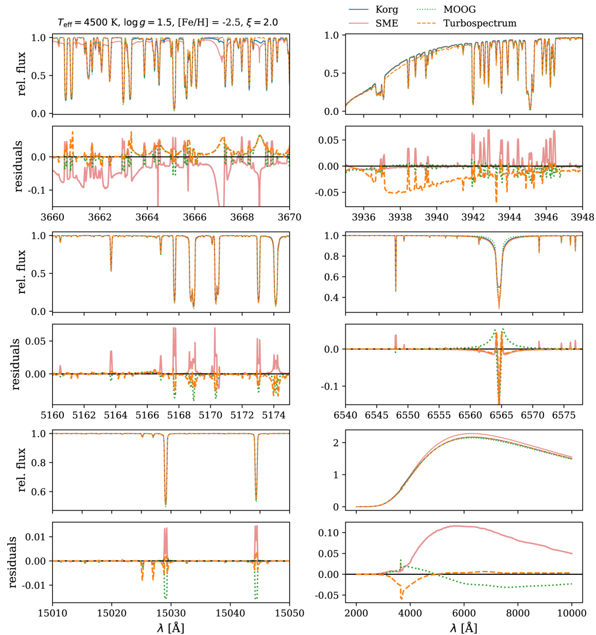
Figure 7. from Adam J. Wheeler et al 2023 Astron. J. 165 doi:10.3847/1538-3881/acaad https://dx.doi.org/10.3847/1538-3881/acaad © 2023. The Author(s). Published by the American Astronomical Society.
