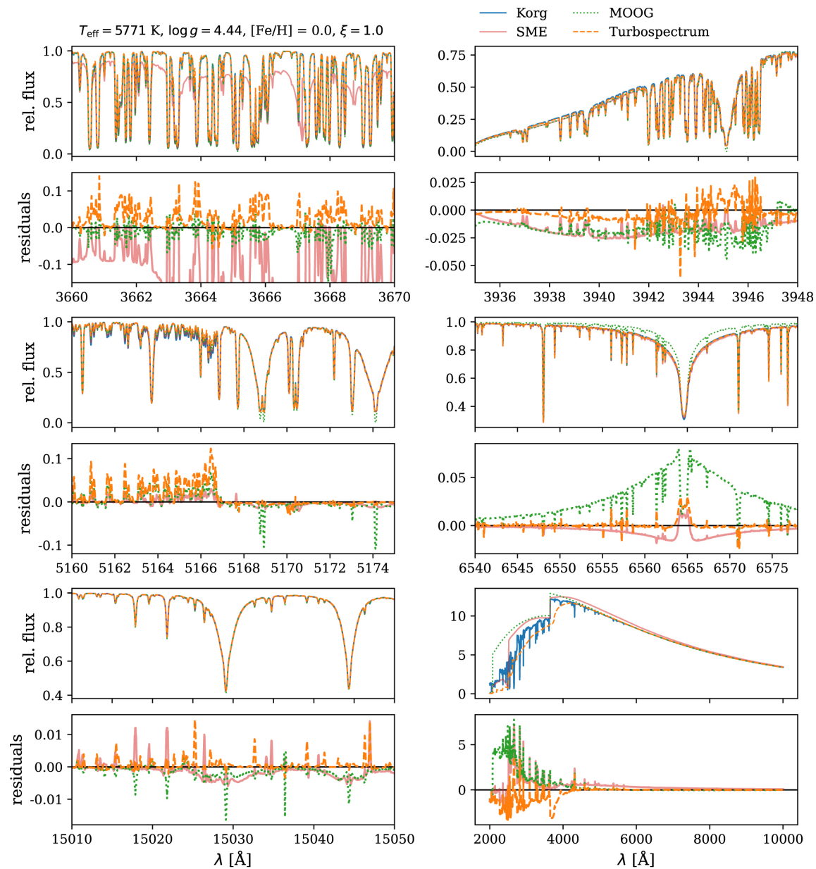
Figure 5. from Adam J. Wheeler et al 2023 Astron. J. 165 doi:10.3847/1538-3881/acaad https://dx.doi.org/10.3847/1538-3881/acaad © 2023. The Author(s). Published by the American Astronomical Society.
