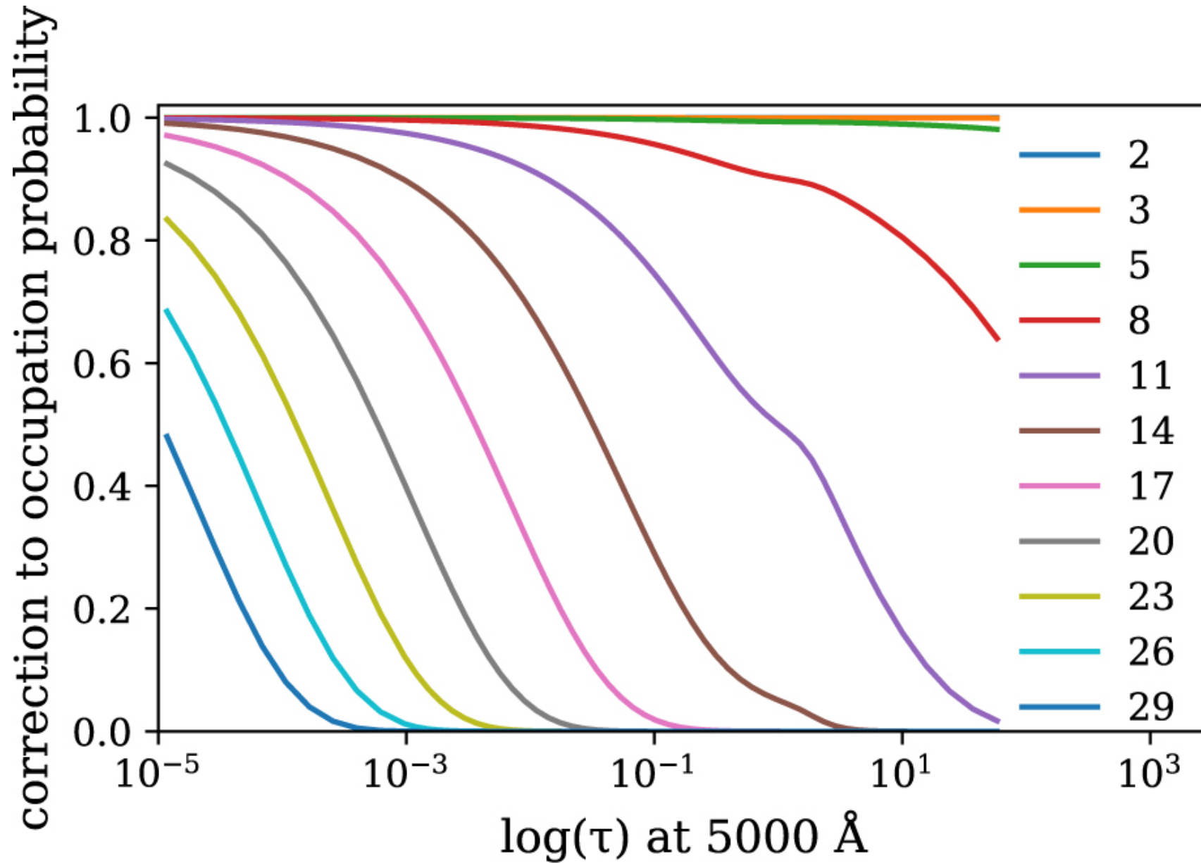
Figure 2. from Adam J. Wheeler et al 2023 Astron. J. 165 doi:10.3847/1538-3881/acaaad https://dx.doi.org/10.3847/1538-3881/acaaad © 2023. The Author(s). Published by the American Astronomical Society.
