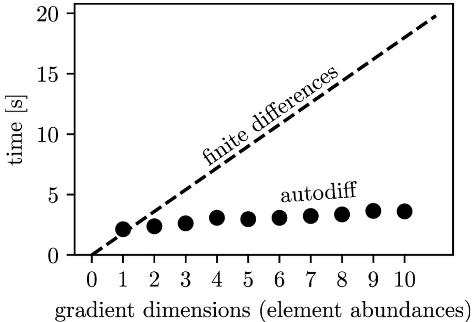
Figure 12. from Adam J. Wheeler et al 2023 Astron. J. 165 doi:10.3847/1538-3881/acaad https://dx.doi.org/10.3847/1538-3881/acaad © 2023. The Author(s). Published by the American Astronomical Society.
