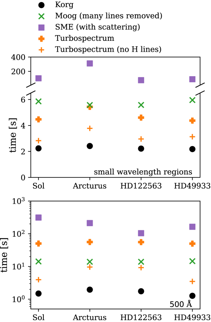
Figure 11. from Adam J. Wheeler et al 2023 Astron. J. 165 doi:10.3847/1538-3881/aaaaad https://dx.doi.org/10.3847/1538-3881/aaaaad © 2023. The Author(s). Published by the American Astronomical Society.
